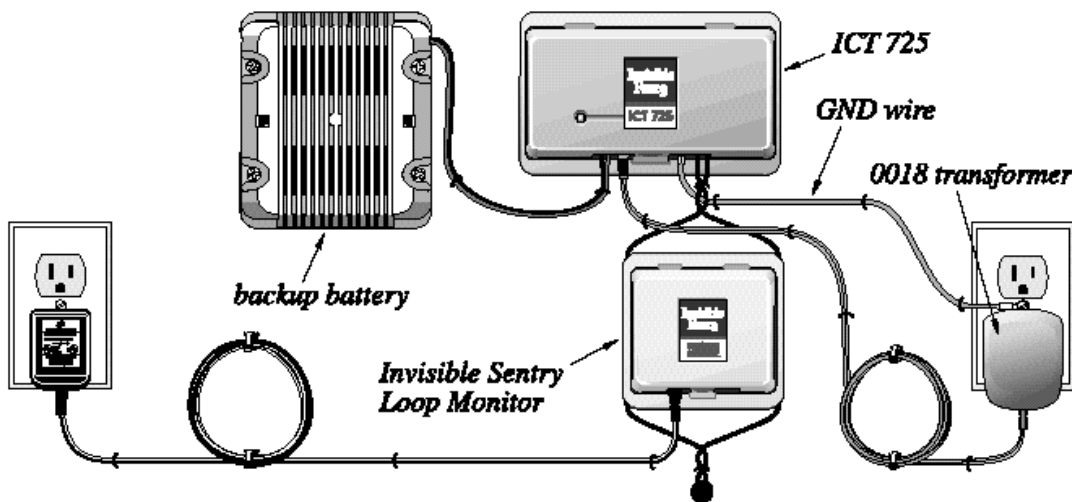
ICT 725 system with a backup battery and an Invisible Sentry™ system.
